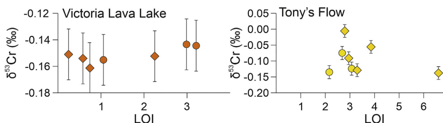
Fig. 6. \delta^{53}\text{Cr} plotted against loss on ignition (LOI) used as an indicator of serpentinisation, for (a) Victoria's Lava Lake and (b) Tony's Flow. No correlations are seen.
